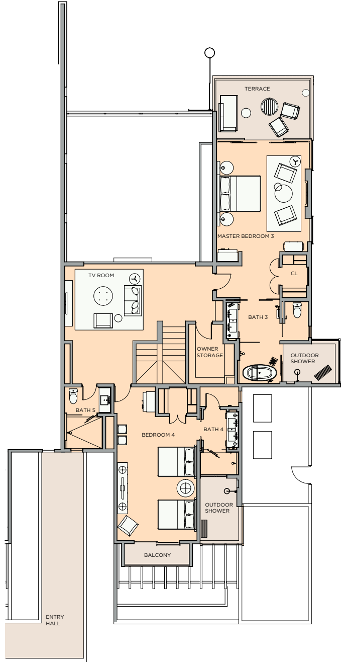
ARCHITECTURAL PLAN LEVEL 2
